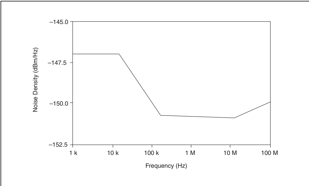
Figure 4. Representation of NI 5124 Spectral Noise Density on 0.2 V Range, Full Bandwidth, 50 \Omega Input Impedance
